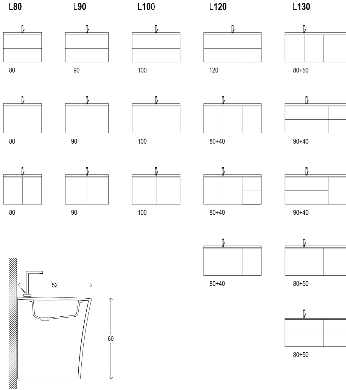
H60 piano curvo | curved plane | plan courbe | gebogene fläche | encimera curva | ИЗОГНУТАЯ СТОЛЕШНИЦА
