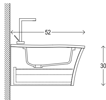
H30 piano curvo | curved plane | plan courbe | gebogene fläche | encimera curva | ИЗОГНУТАЯ СТОЛШНИЦА
